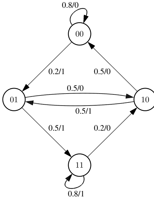
Figure 2-2. State diagram of a second-order Markov source with alphabet \{0, 1\}
